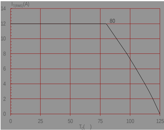
FIG.4: On-state characteristics
