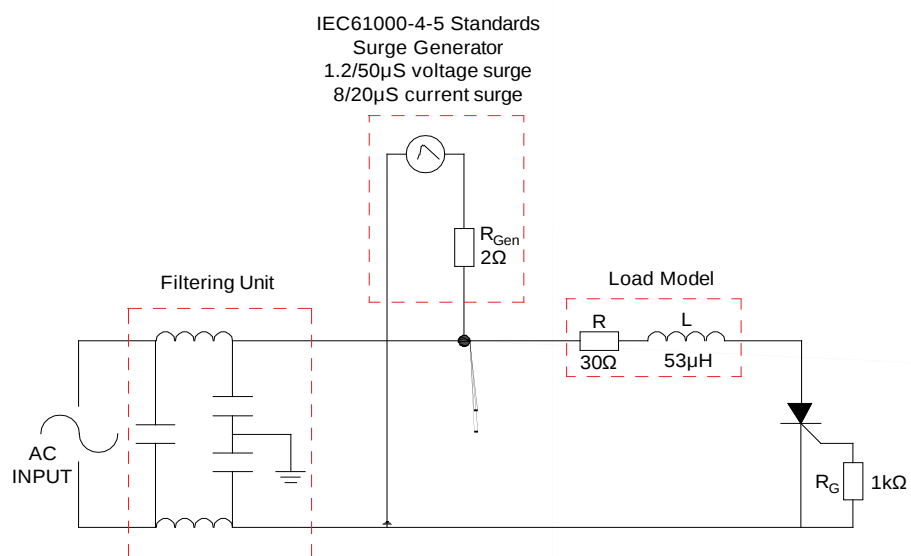
FIG 8 Test circuit for inductive and resistive loads to IEC-61000-4-5 standards. SOLDER
