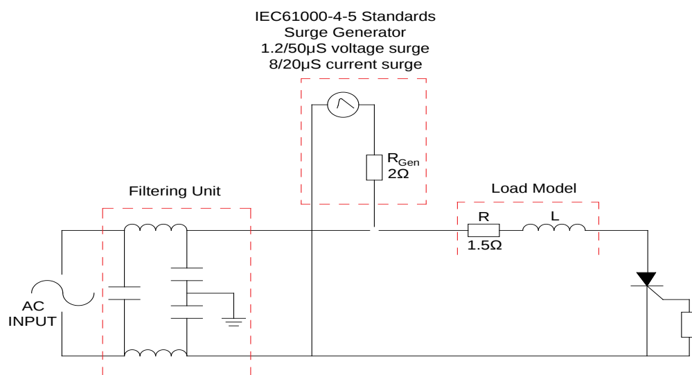
FIG.7 Test circuit for inductive and resistive loads to IEC-61000-4-5 standards. S
